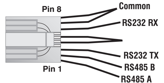
RS232/RS485 Pin-Out (Shown Tab-side Up)
